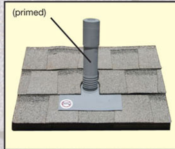
Adjustable Lead Flashing Available with or without Cap. Shown with Cap.
